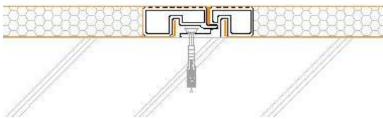
Option 1 - Direct fix to wall
