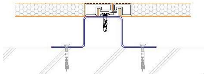
Option 2 - Batten fix to wall
